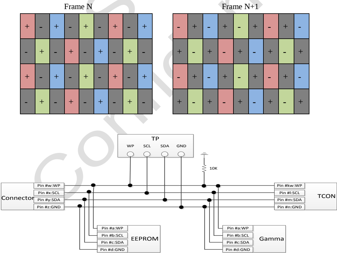
Fig 4.8 Flicker adjust circuit block diagram
