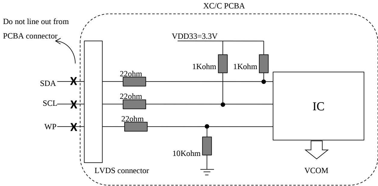
Fig. 4.3 WP/SDA/SCL PCBA set
