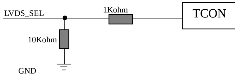
Fig. 4.4 LVDS_SEL PCBA set
