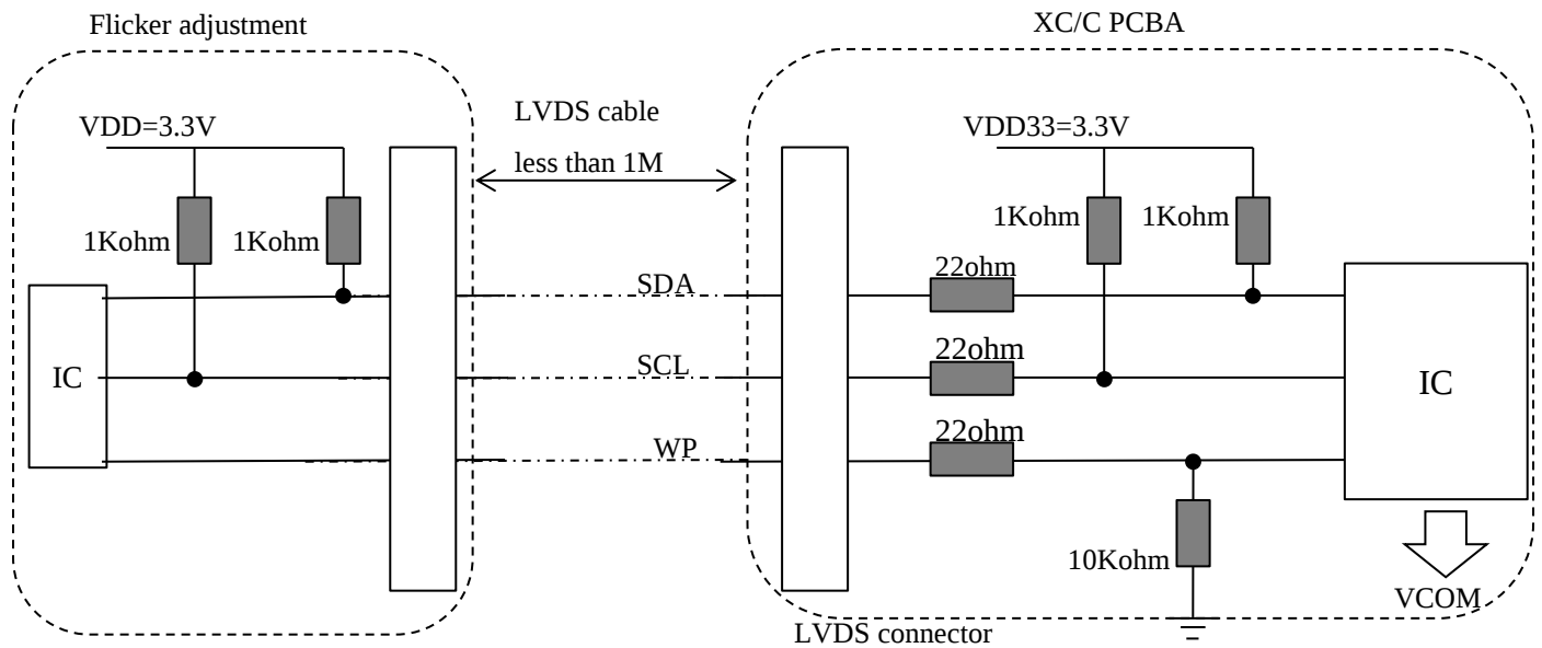
Fig. 4.4 WP/SDA/SCL flicker set
