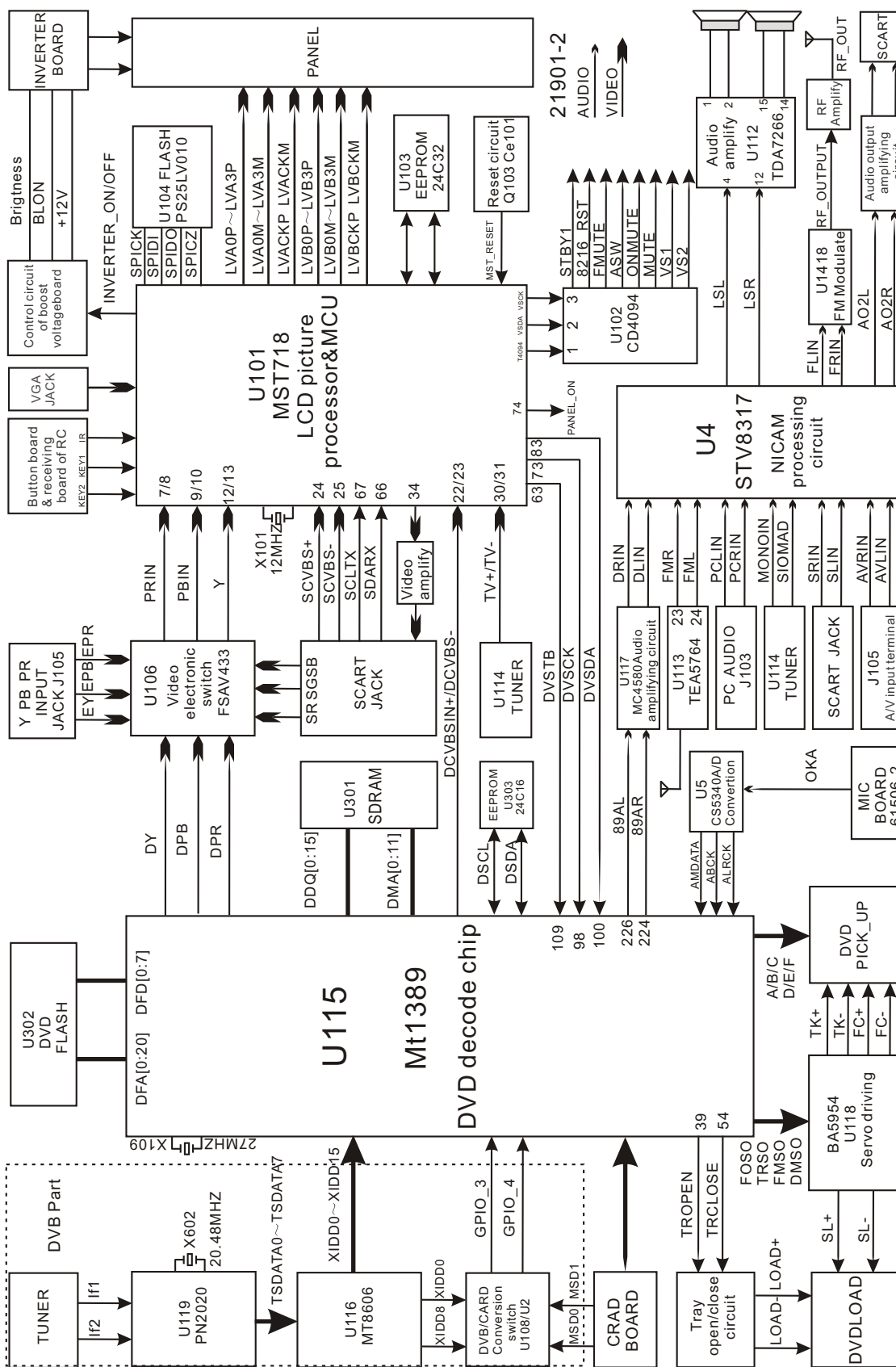
figure 3.1.3.1 Block diagram of the player
