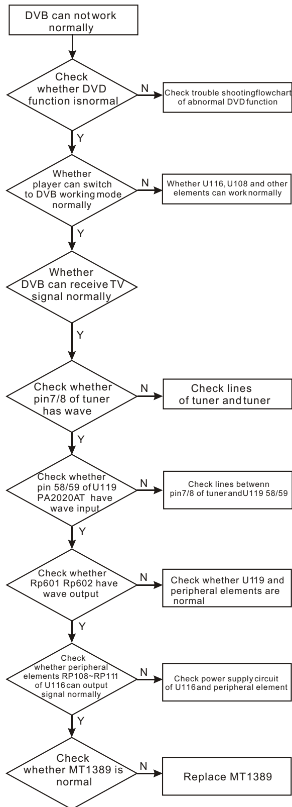
[ Flow chart 14 ]Symptom: “Troubleshooting flow chart of DVB module”
