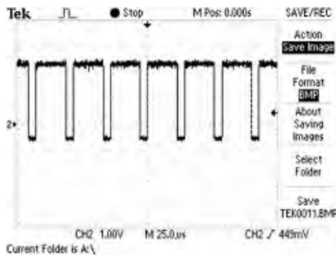
16. CN1_12 display screen enable control end waveform diagram
