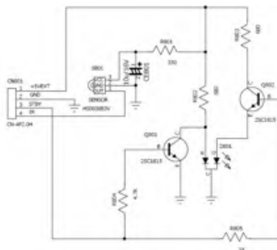
Figure 3.2.1.6 Working state indication circuit diagram
