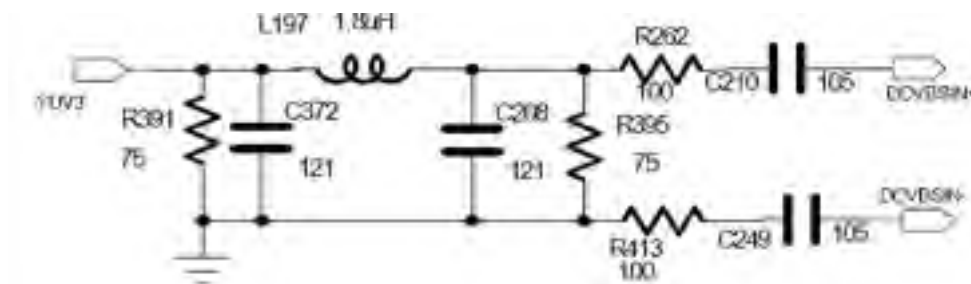
Figure 3.2.10.2 Video output circuit
