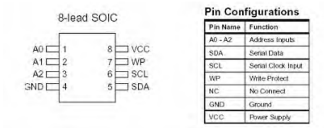
Figure 3.5.5.1 Casing and pin function explanation
