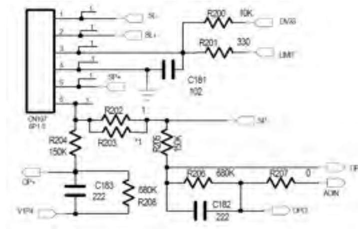
Figure 3.2.7.1 Main axis control circuit diagram
