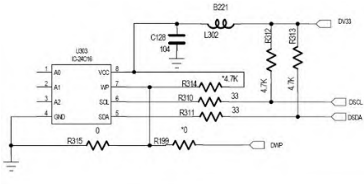
Figure 3.5.5.2 Circuit schematic diagram
