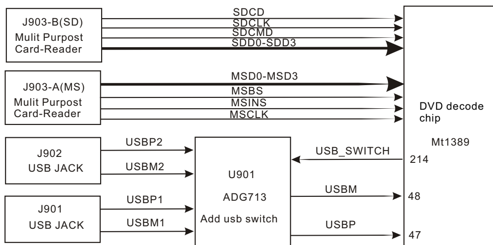
Figure 3.2.12.1 usb/card circuit diagram
