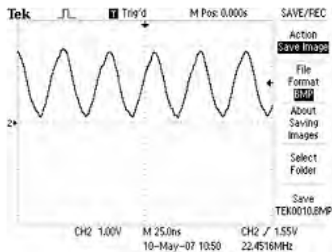
15. CN1_11 display screen drive clock signal waveform diagram
