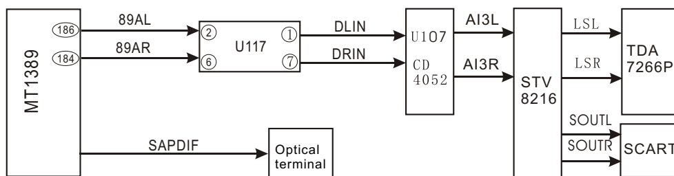
Figure 3.2.11.1 Audio signal flow chart block diagram
