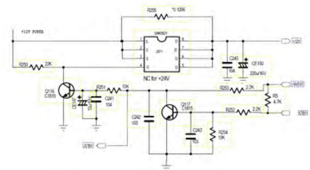
Figure 3.2.5.4 +12V Power control circuit diagram
