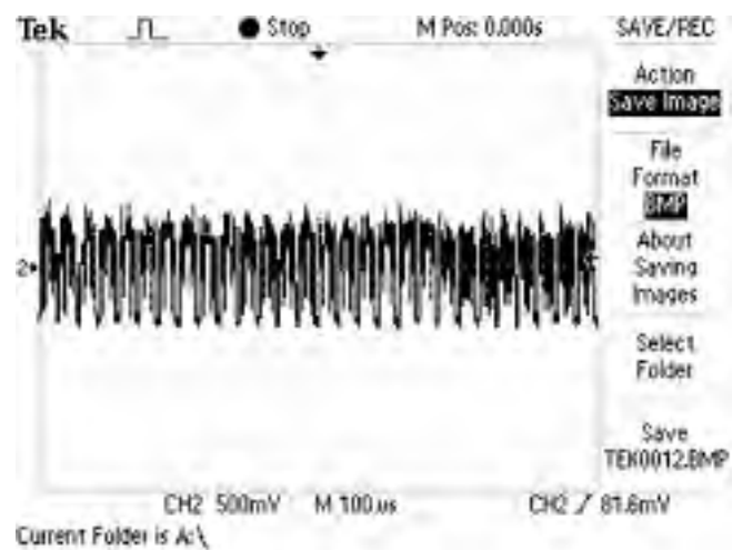
17. CN1_12 waveform diagram of VSYNC signal outputted by MST718
