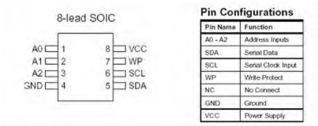
Figure 3.5.5.1 Casing and pin function introduction
