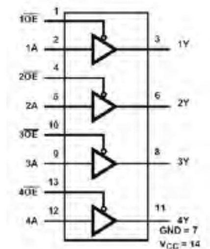
Figure 3.5.6.1 Truth value table and 74HCT125 function module structure
