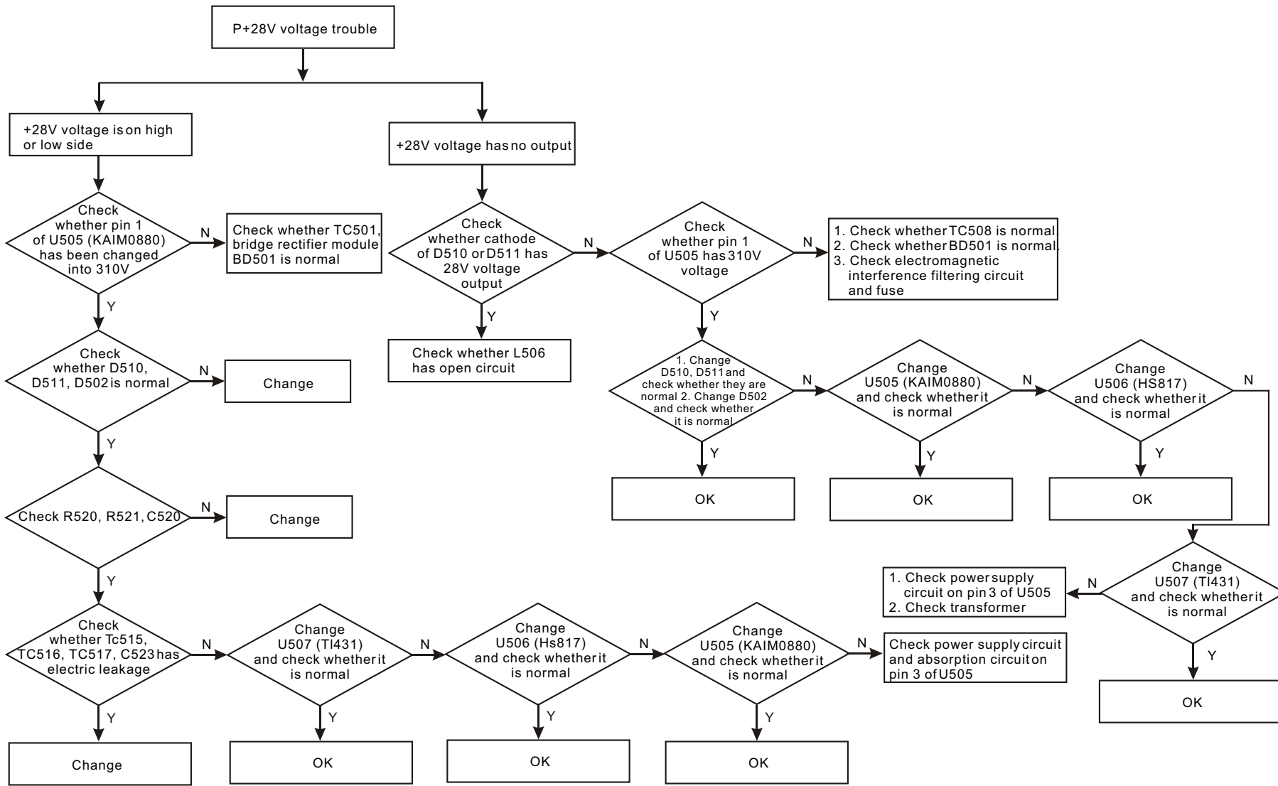
16. Troubleshooting process for P+28V voltage is shown as the following figure 3.3.2.17:
