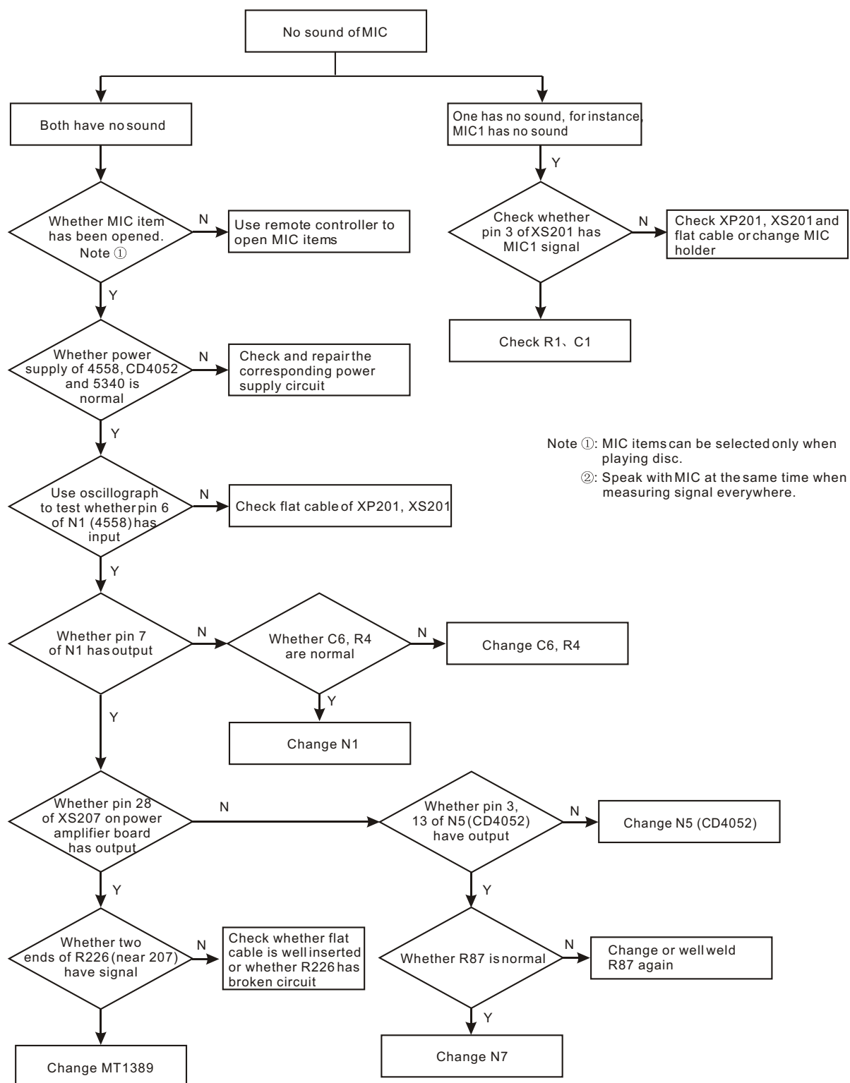
Figure 3.3.2.8 Troubleshooting flow chart for no sound of MIC
