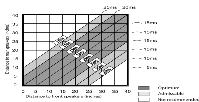
Fig. 2. Determine delay value as to Dolby Pro Logic mode.
