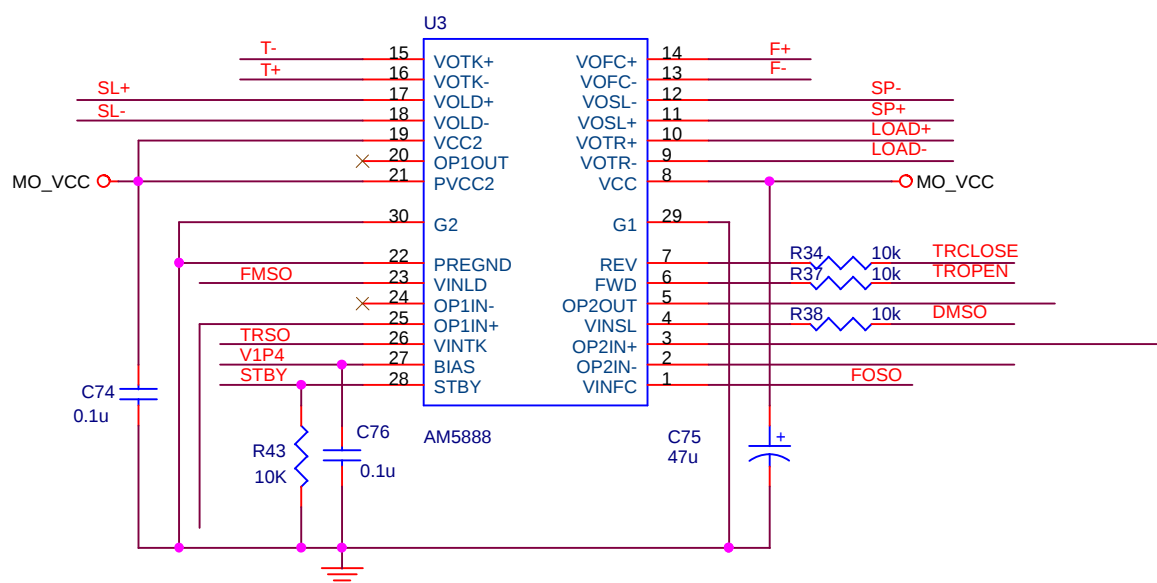
Figure 3.2.4.1 Open/close door circuit diagram
