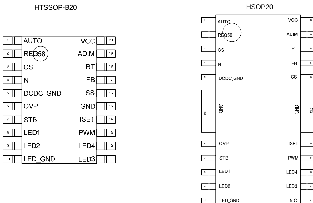
Figure 3. Pin Configuration
