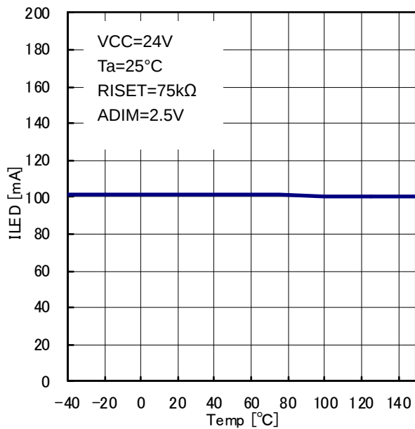
Figure 9. LED Current ( I_{LED} ) [mA] vs. Temp [ ^\circ\text{C} ]
